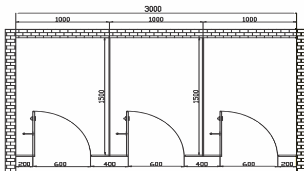
Top View (EU)
