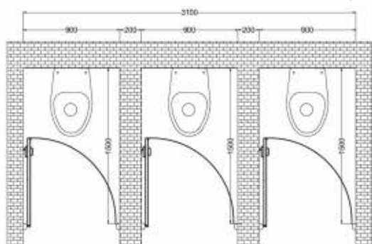
Top View (EU)
